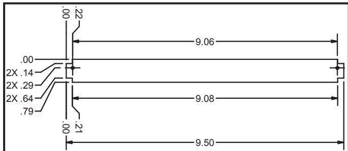
Twin Cam Handle Front Panel Cutouts
