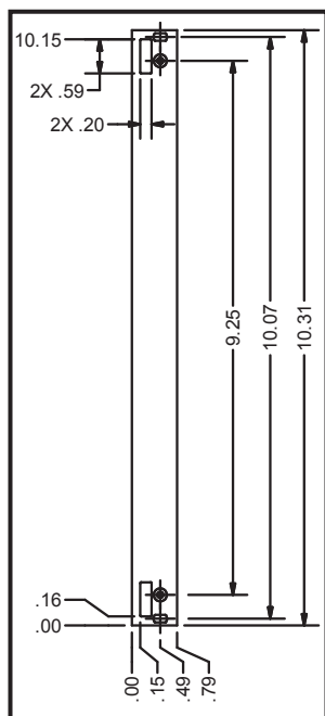
Twin Cam Handle Front Panel Cutouts
